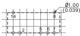
RECOMMENDED FOOTPRINT Top view, grid: 2.54*2.54mm (0.1*0.1inch)
